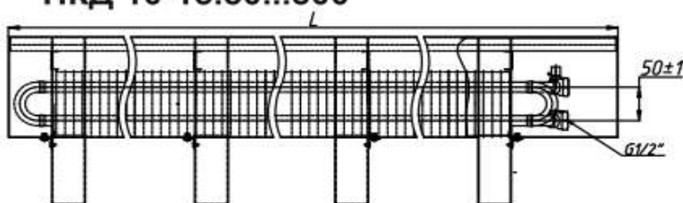
НКД 10-15.50...300
